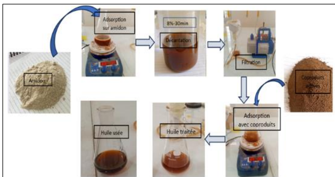
Figure 8 Steps in the oil purification process
