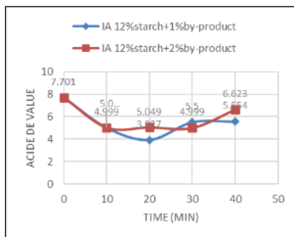
Figure 15 Acide value with starch (12%) and 1/2% ATBp)
