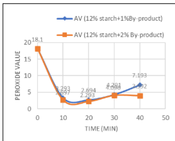
Figure 13 Peroxide value with starch (12%) and 1/2% ATBp)
