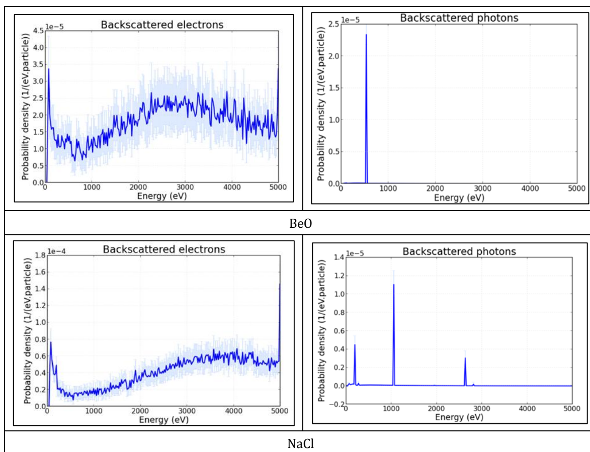
Figure 1 Probability density of backscattered particles as a function of energy
